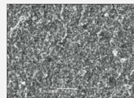
Yestool's New carbide material (0.2+0.5+0.8 \mu m ultra-micro grain size)
