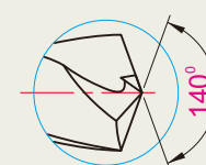
Standard Point
