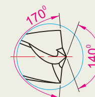
"F" Flatted Point
