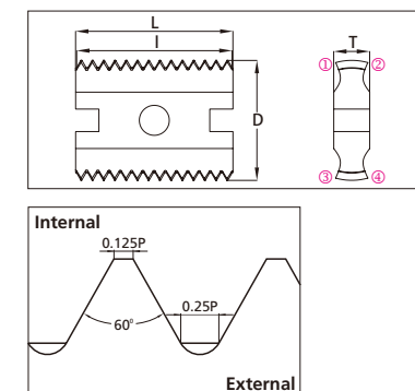
ITM Carbide Thread mill inserts
